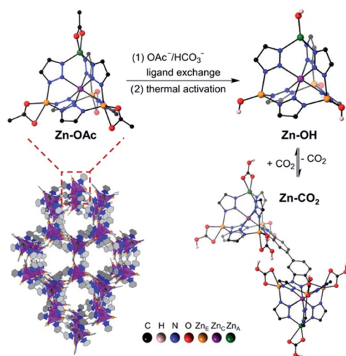
Fig. 3 Crystal structure of a \text{Zn} -benzotriazolate MOF functionalized with \text{Zn-OH} binding sites and reaction with \text{CO}_2 . Reproduced with permission from ref. 32. Copyright (2020) American Chemical Society.
