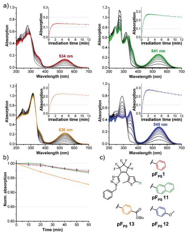
Fig. 5 Photochromic properties of various thieryl substitutions: (a) time-dependent changes of the absorption spectra of 60 \mu\text{M} solutions of pF PS 1, 11–13 upon UV light irradiation (310 nm, LED) in chloroform towards the (pseudo)-photostationary state; insets show the absorption vs. time trace measured at the VIS absorption maximum during extended UV irradiation to analyse the photostability, (b) thermostability (20 °C) of the CF isomers, (c) structures.
