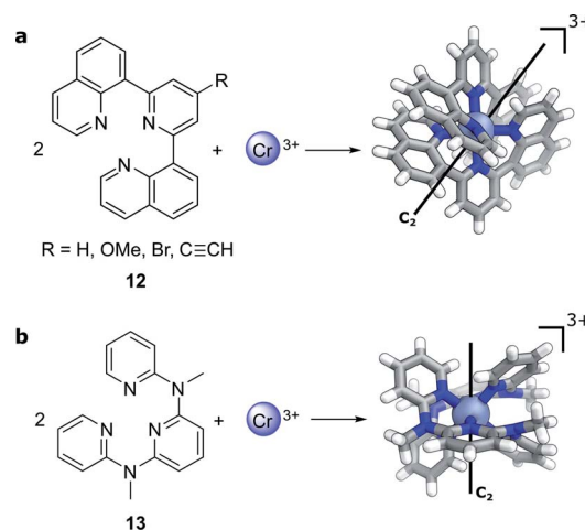
Fig. 6 The crystal structure of two Cr(III) complexes displaying |g_{\text{lum}}| values of (a) 0.2 ( \text{R} = \text{H} , ref. 44; \text{R} \neq \text{H} , ref. 46) and (b) 0.093 (ref. 45).
