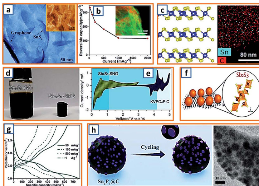
Fig. 15 Potassium storage chemistry and applications of anodes with conversion–alloy mechanism. (a) Microstructure of obtained \text{SnS}_2@r\text{GO} composite. Reproduced with permission. 5 Copyright 2019, Wiley. (b) Electrochemical performance of \text{SnS}_2 -rGO composite with an energy-filtered TEM image (color scheme: red-sulfur, green-carbon) inserted. Reproduced with permission. 38 Copyright 2017, The Royal Society of Chemistry. (c) Schematic crystal structure of \text{SnS}_2 in N, S-C/ \text{SnS}_2 NSs, and its corresponding elemental mappings. Reproduced with permission. 60 Copyright 2020, Elsevier. (d) Photographs of the \text{Sb}_2\text{S}_3 -GO precursor solution and \text{Sb}_2\text{S}_3 -SNG composite and (e) CV curves of \text{Sb}_2\text{S}_3 -SNG/KVPO 4 F-C full cells. Reproduced with permission. 73 Copyright 2017, Springer. (f) Schematic representation of the nanocrystalline \text{Sb}_2\text{S}_3 coated by rGO NSs, and (g) charge/discharge curves at various current densities. Reproduced with permission. 93 Copyright 2020, The Royal Society of Chemistry. (h) Illustration of the potassium storage behavior of the \text{Sn}_4\text{P}_3@C active material. Reproduced with permission. 105 Copyright 2019, Elsevier.
