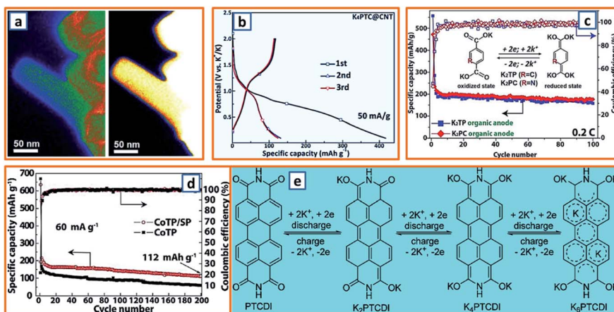
Fig. 18 Potassium storage chemistry and applications of organic anodes. (a) EELS spectra of ADAPTS organic compound at low (left) and high (right) energy loss regimes. Reproduced with permission. 12 Copyright 2018, Wiley. (b) Charge–discharge curves of K_4 PTC@CNT anode during the three initial cycles. Reproduced with permission. 29 Copyright 2019, The Royal Society of Chemistry. (c) Long cycle profiles of K_2 TP and K_2 PC organic anodes for 100 cycles. Reproduced with permission. 51 Copyright 2017, Elsevier. (d) Cycling performance of CoTP and CoTP/super P in K-ion cells ( 60 \text{ mA g}^{-1} ). Reproduced with permission. 72 Copyright 2017, Elsevier. (e) Possible six-electron storage mechanism for organic PTCDI anode. Reproduced with permission. 86 Copyright 2019, The Royal Society of Chemistry.
