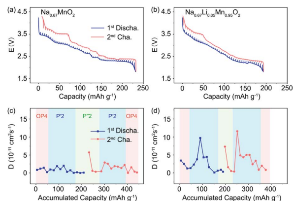
Fig. 5 GITT profiles of (a) \text{P'2-Na}_{0.67}\text{MnO}_2 and (b) \text{P'2-Na}_{0.67}\text{Li}_{0.05}\text{Mn}_{0.95}\text{O}_2 in a charge and discharge cycle. \text{Na}^+ diffusion coefficients of (c) \text{P'2-Na}_{0.67}\text{MnO}_2 and (d) \text{P'2-Na}_{0.67}\text{Li}_{0.05}\text{Mn}_{0.95}\text{O}_2 calculated from GITT measurements.
