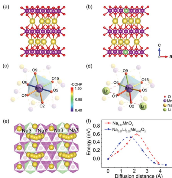
Fig. 4 Optimized structure of (a) \text{P'2-Na}_{0.67}\text{MnO}_2 and (b) \text{P'2-Na}_{0.67}\text{Li}_{0.05}\text{Mn}_{0.95}\text{O}_2 . COHP analysis of the transition metal octahedral sites of (c) \text{P'2-Na}_{0.67}\text{MnO}_2 and (d) \text{P'2-Na}_{0.67}\text{Li}_{0.05}\text{Mn}_{0.95}\text{O}_2 . (e) Na3–Na7 diffusion pathway in \text{P'2-Na}_{0.67}\text{Li}_{0.05}\text{Mn}_{0.95}\text{O}_2 . (f) activation energy barrier for \text{Na}^+ diffusion in \text{P'2-Na}_{0.67}\text{MnO}_2 and \text{P'2-Na}_{0.67}\text{Li}_{0.05}\text{Mn}_{0.95}\text{O}_2 .
