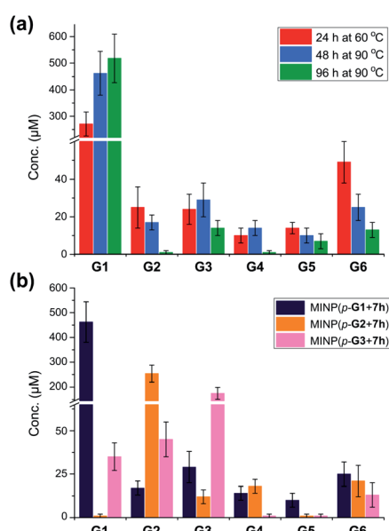
Fig. 1 (a) Product distributions for the hydrolysis of 100 μM maltohexaose ( G6 ) under different conditions using 20 μM MINP( p -G1 + 7h) in 10 mM MES buffer (pH 6). (b) Product distributions for the hydrolysis of 0.1 mM maltohexaose ( G6 ) using different MINPs (20 μM) in 10 mM MES buffer (pH 6) at 90 °C for 48 h. See Table S4† for the exact numbers.
