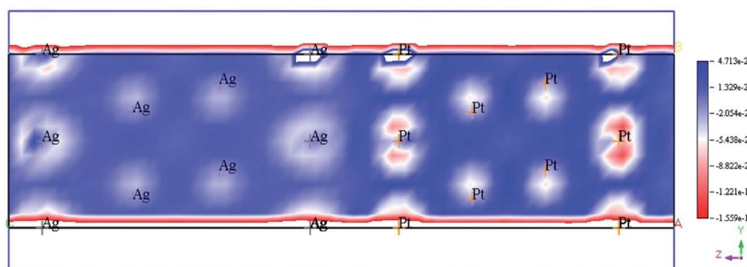
Fig. 19 Electron deformation density of the 2 x 2 layer of Pt (111) and Ag (111) surfaces, and the loss and gain of electrons are indicated in blue and red, respectively. This figure is reproduced from ref. 138 with permission from Elsevier, copyright 2017.
