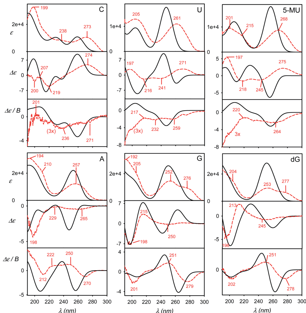
Fig. 3 Calculated (black, solid) and experimental (red, dashed) absorption ( \epsilon ), ECD ( \Delta\epsilon ) and MCD ( \Delta\epsilon/B ) spectra of six nucleosides, a B3LYP/6-311+G**/CPCM weighted average over six geometries representing minima I–VI defined in Fig. 2 and S2.†
