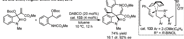
Scheme 85 Reaction of MBH carbonates with \pi -allyl precursors.
