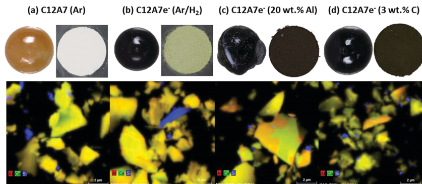
Fig. 2 Top: Pictures of ingots obtained after plasma treatment and powders after grinding of the ingots; bottom: EDX maps of TEM studies of (a) pure C12A7 treated under Ar atmosphere, (b) pure C12A7 treated under 95% Ar/5% H 2 atmosphere, (c) 20 wt%-Al/C12A7 mixture treated under 95% Ar/5% H 2 and (d) 3 wt%-C/C12A7 mixture treated under 95% Ar/5% H 2 . The EDX images show the distribution of Al (red), Ca (green) and the ratio (yellow to orange) of both. Si (blue) is present due to TEM sample preparation. Orange areas are assigned to CA (krotite) secondary phase and yellow areas to C12A7 based on different Ca to Al ratios in the two phases.
