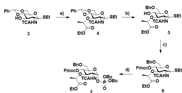
Scheme 2 Synthesis of the MurNAC BB 2. Reagents and conditions: (a) (–)-ethyl (S)-2-trifluoromethylsulfonyl propionate, NaH, DMF/CH 2 Cl 2 , 0 °C → rt, 53%; (b) Me 3 N·BH 3 , BF 3 ·OEt 2 , CH 3 CN, 0 °C → rt, 65%; (c) FmocCl, pyridine, CH 2 Cl 2 , rt, 93%; (d) (BuO) 2 P(O)OH, NIS, TfOH, 0 °C → rt, 83%.
