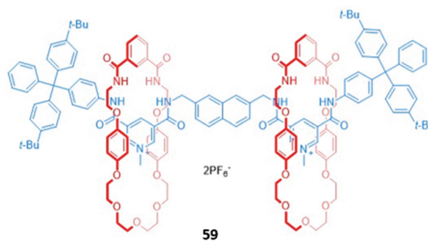
Fig. 33 A dicationic [3]rotaxane which displays an unusual optical response to \text{SO}_4^{2-} ( K_1 > 10^4 \text{ M}^{-1} in 45 : 45 : 10 \text{CDCl}_3/\text{CD}_3\text{OD}/\text{D}_2\text{O} ).
