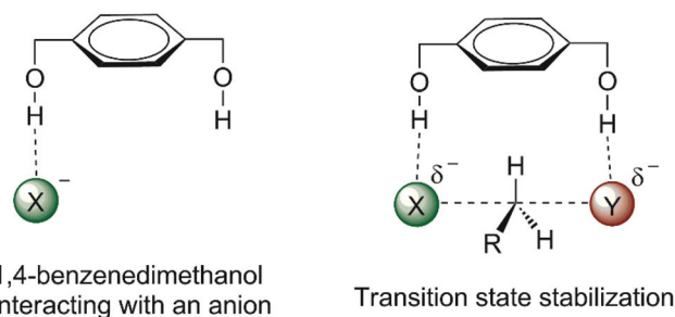
Fig. 6 Envisioned catalytic effect in S_N2 reactions by hydrogen bonds to the incoming and leaving groups.
