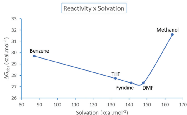
Fig. 5 Observed effective free energy barrier for the TMAF + ArBr reaction as a function of the solvation free energy (absolute values) of the pair of ions N(CH_3)_4^+ + F^- . Theoretical values. 40
