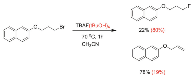
Scheme 4 Fluorination with anhydrous TBAF (black) and with the complex TBAF(tBuOH)_4 (red).
