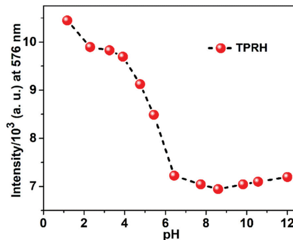
Fig. 4 Fluorescence response of TPRH at 576 nm (20 \mu M, \lambda_{\text{ex}} = 350 nm) as a function of pH in \text{CH}_3\text{OH}-\text{H}_2\text{O} (1 : 4, v/v, 25 ^\circ\text{C} ); the pH was adjusted by using 1 M HCl or 1 M NaOH aqueous solution.
