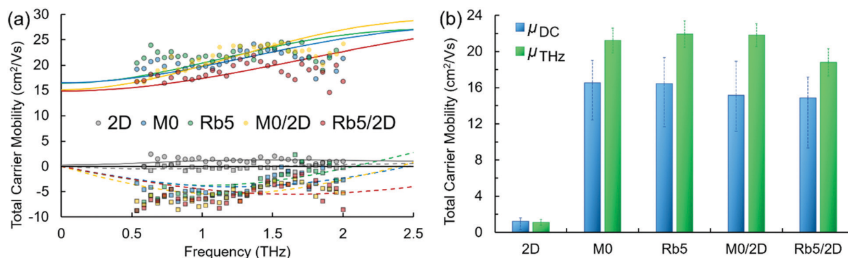
Fig. 5 TRTS data collected using 1.25 \text{ mJ cm}^{-2} , 400 nm photoexcitation and a 5 ps time delay between UV photoexcitation and the THz probe. (a) Frequency-dependent complex TRTS responses for 2D layered \text{PEA}_2\text{PbI}_4 , 3D M0 and Rb5, and 3D/2D heterostructure perovskite solid-state films. Circles/solid line fits and squares/dashed line fits represent the total mobility's real and imaginary components (converted from the photoinduced dielectric response), respectively. (b) Resulting \mu_{DC} (zero-frequency limit of the real mobility in (a)) and \mu_{THz} (average of the real part over the data range of 0.5 THz to 2 THz) extracted for each dataset. The error bars in (b) indicate 95% confidence intervals (type A k = 1.96 analysis) for each extracted mobility value.
