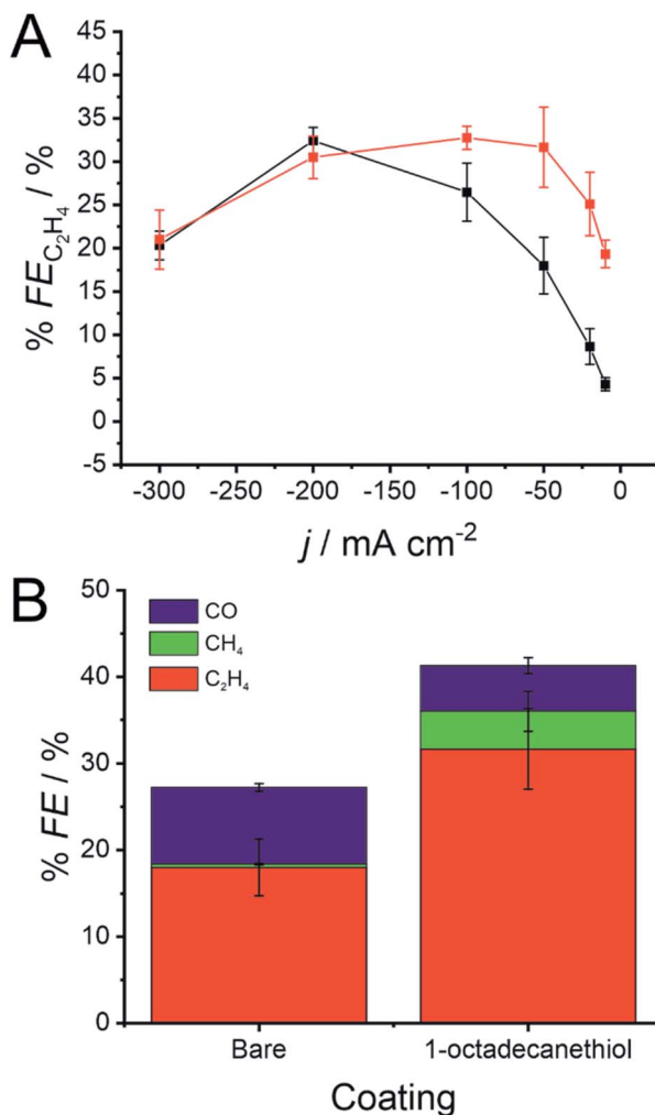
Fig. 4 (A) Faradaic efficiency for \text{C}_2\text{H}_4 formation (% \text{FE}_{\text{C}_2\text{H}_4} ) during galvanostatic \text{CO}_2 reduction at a 500 nm Cu GDE in 1 M KOH with (red) and without (black) a monolayer of 1-octadecanethiol to form a hydrophobic interface. (B) % FE for CO, \text{CH}_4 and \text{C}_2\text{H}_4 with and without the 1-octadecanethiol layer during galvanostatic \text{CO}_2 reduction at -50 \text{ mA cm}^{-2} using the same conditions as in (A). Error bars display one standard deviation ( n = 3 ).
