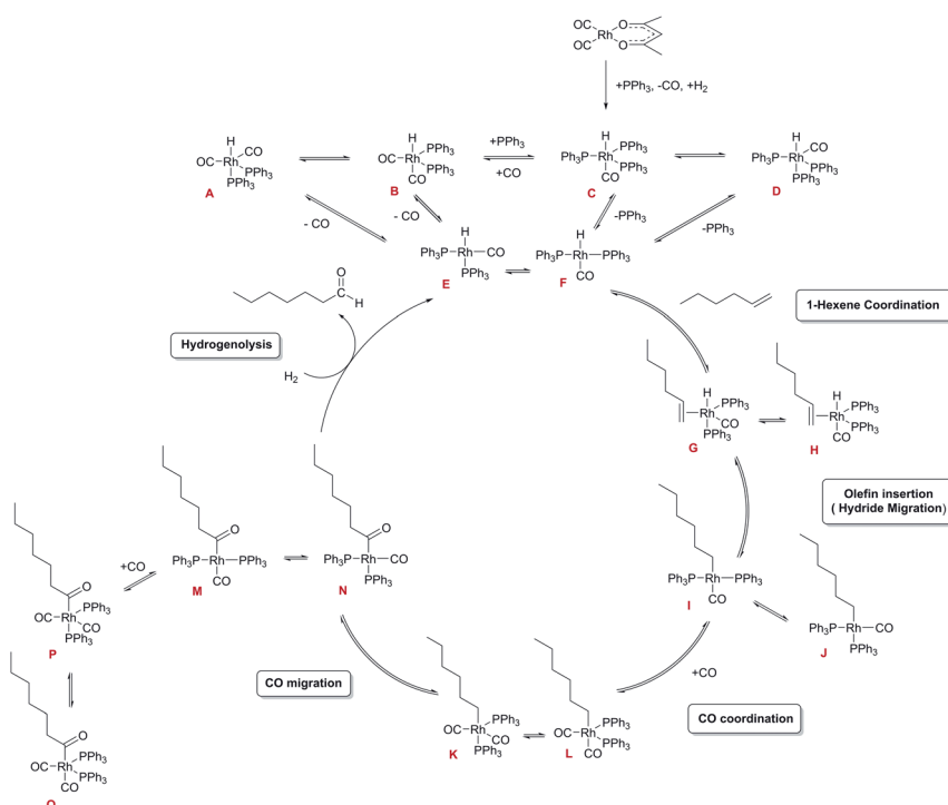
Scheme 2 Simplified dissociative mechanism for the Rh-catalysed hydroformylation of hexene (only heptanal formation shown). All in-cycle reaction intermediates are believed to contain two PPh 3 ligands per Rh.
