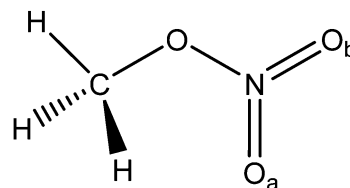
Scheme 1 Molecular structure of \text{CH}_3\text{ONO}_2 .
