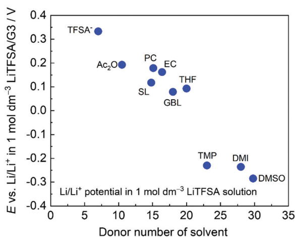
Fig. 4 \text{Li}/\text{Li}^+ potential in 1 \text{ mol dm}^{-3} LiTFSA in different solvents plotted against donor number of each solvent, measured at 30 °C. TFSA - indicates 1 \text{ mol dm}^{-3} LiTFSA/[P13][TFSA]. [P13][TFSA]: N -Methy- N -propylpyrrolidinium bis(trifluoromethanesulfonyl)amide, Ac 2 O: acetic anhydride, TMP: trimethyl phosphate, and DMI: 1,3-dimethyl-2-imidazolidinone. Reference electrode: \text{Li}/\text{Li}^+ in 1 \text{ mol dm}^{-3} LiTFSA/G3.
