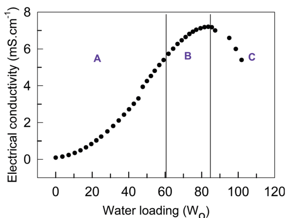
Fig. 7 Electrical conductivity ( \text{mS cm}^{-1} ) as a function of water loading ( w_o ) in water/TX-100 (300 mM)/TBAC-DA microemulsion at ambient conditions. Regions A, B, and C are described in the text.
