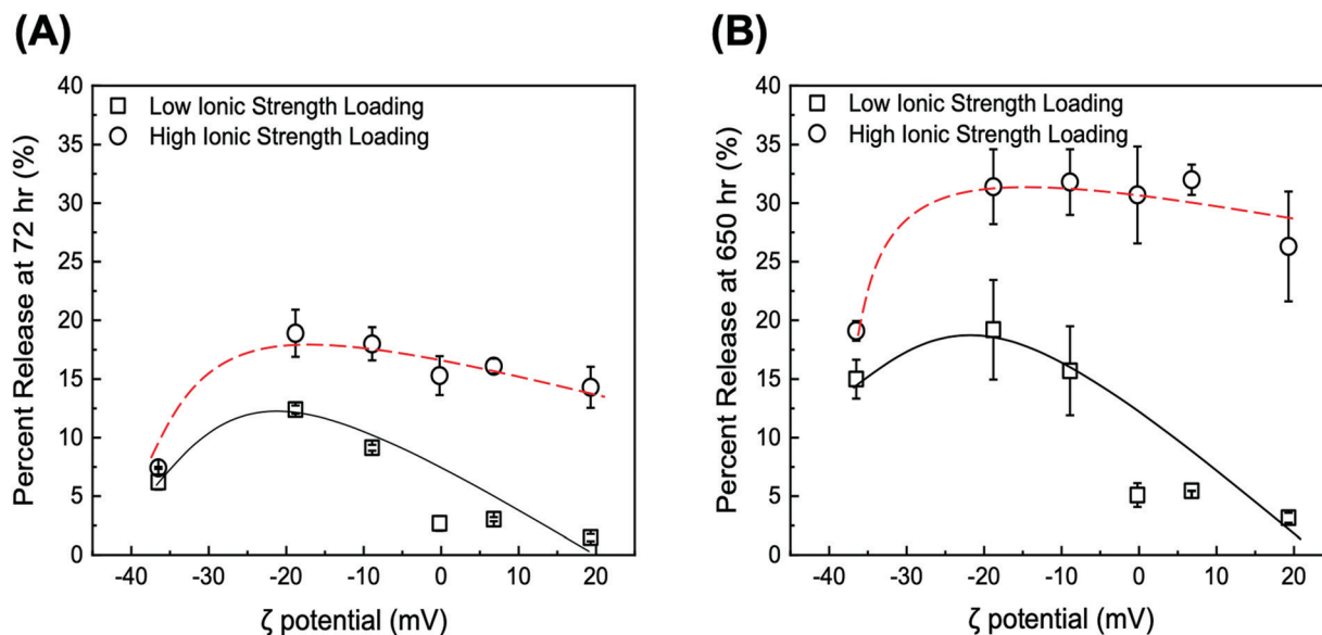
Fig. 6 Values of DOX percent release at pH 5 after (A) 72 h and (B) 650 h from DOX/GO and DOX/tGO particles loaded at neutral pH and low ionic strength (squares) or high ionic strength (circles). Shaded are added to guide the visualization of the results. Error bars represent mean \pm 99% CI ( n \geq 3 ).
