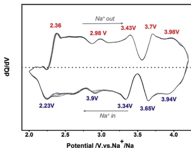
Fig. 17 Differential capacity ( dQ/dV ) vs. potential ( V ) of \text{P2-Na}_{2/3}\text{Co}_{1/2}\text{Ti}_{1/2}\text{O}_2 , cycled vs. \text{Na/Na}^+ in an electrochemical half-cell. Reproduced with permission from ref. 240.
