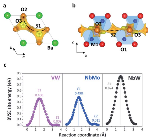
Fig. 7 BVSE map of Ba 3 VWO 8.5 showing the 2-dimensional ionic conduction pathway along the palmierite-like layer as seen down the c -axis (a) and a -axis (b). Isosurface levels are drawn at < 0.5 eV (over the global minimum). The dotted lines represent the saddle points as identified by the softBV software. (c) BVSE models of migration barriers along the palmierite-like layers for Ba 3 VWO 8.5 (VW), Ba 3 NbMoO 8.5 (NbMo), and Ba 3 NbWO 8.5 (NbW). Relative bond-valence energy barriers are reported in eV. Note that the minimum site energies have relative values.
