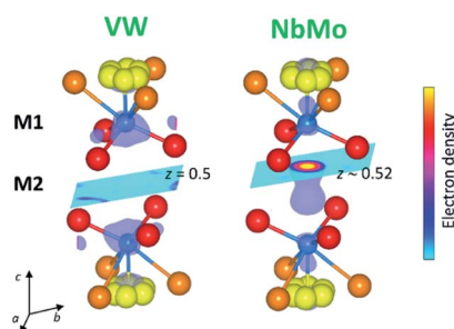
Fig. 4 Volumetric data obtained from the X-ray difference Fourier analysis on the refined structures of Ba 3 VWO 8.5 (VW) and Ba 3 NbMoO 8.5 (NbMo). The difference Fourier map for Ba 3 VWO 8.5 shows no evidence of electron density on or in proximity of the 3 b (0,0,0.5) M2 site. In contrast the map for Ba 3 NbMoO 8.5 , calculated by setting the occupancy of M2 to zero, clearly indicates missing electron density located for the most part at the 6 c (0,0,~0.52) site. Sections represent slices of the volumetric Fourier data seen along the [001] direction at z = 0.5 (VW) and at z \sim 0.52 (NbMo). The metal cations are represented by the blue spheres, while the oxygen atoms are in red (O1), orange (O2) and yellow (O3).
