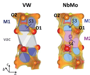
Fig. 8 Bond-valence site energy maps calculated for Ba 3 VWO 8.5 (VW) and Ba 3 NbMoO 8.5 (NbMo). The cation vacancy (vac) in VW is represented by the grey octahedron. The dotted lines represent the saddle points at the median of the O1–O2 (S3) and O1–O1 (S4) distances, with bottlenecks constituted by triangles formed by two Ba cations and one M cation, as identified by the softBV software. Darker colours indicate the lower isosurface levels (<0.5 eV over the global minimum), while the lighter colours are for the highest isosurface levels (between 0.7 eV and 1.4 eV over the global minimum).
