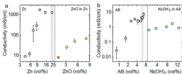
Fig. 2 (a) The conductivity of semi-solid electrodes with different volume percentages of Zn particles (Zn, 100–300 μm in size, Fig. S2a†), where the conductive percolation threshold was ~5.5 vol%, and the conductivity of anolyte (ZnO in Zn) as a function of volume fraction of ZnO (100–500 nm in size, Fig. S2c†) from 1.1 to 8.1%, accompanied with comparable volume percentages of Zn particles (21.3–22.9 vol%). (b) The conductivity of semi-solid electrodes with different volume percentages of acetylene black (AB, 50–100 nm in particle size, Fig. S2b†) only, where the conductive percolation threshold was ~2.5 vol%, and with different volume percentages of \text{Ni}(\text{OH})_2 (10–30 μm in size, Fig. S2d†) with comparable percentages of AB (5.4–6.1 vol%). The detailed compositions of these suspensions are listed in Tables S1–S4.† The standard deviations were calculated from three independent measurements.
