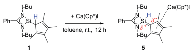
Scheme 5 Synthesis of \{[\text{PhC}(\text{NtBu})_2\text{SiH}(\text{C}_5\text{Me}_4)]\{\text{Ca}(\text{C}_5\text{Me}_5\text{I})\} ( 5 ).
