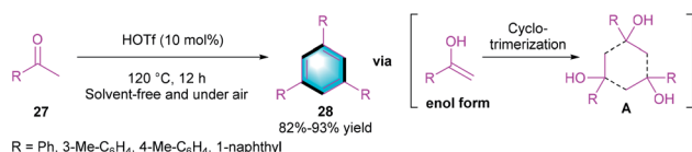
Scheme 7 HOTf-catalyzed [2 + 2 + 2] benzannulation to synthesize tri-substituted arenes.
