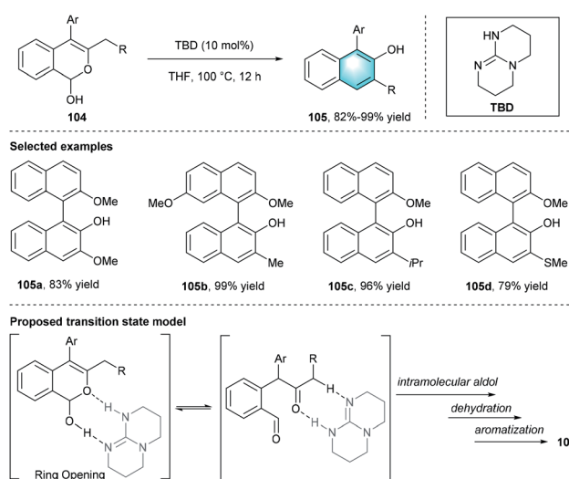
Scheme 29 TBD-catalyzed intramolecular benzannulation to synthesize substituted biaryls.
