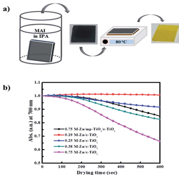
Fig. 3 (a) The decomposition behaviors and (b) the decrease in the absorbance at 700 nm over 600 s of the \text{MAPbI}_3 perovskite film fabricated by this sequential dip-coating deposition on \text{ZnO}/\text{c-TiO}_2 layer observed during solvent drying.
