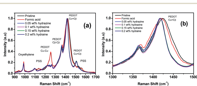
Fig. 7 (a) Raman spectra of the PEDOT:PSS films before and after treatment with formic acid and formic acid-hydrazine. (b) The zoomed spectra for the wavenumbers ranging from 1300 to 1500 \text{cm}^{-1} .
