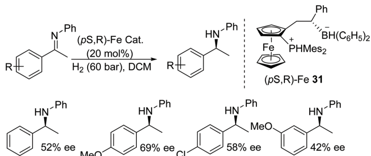
Fig. 42 Iron catalysed AH of N -alkylated imines.
