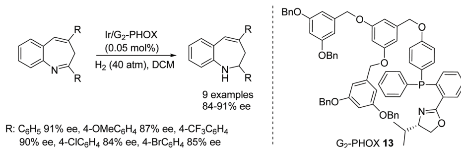
Fig. 18 Chemoselective and enantioselective AH of 2,4-diaryl-3H-benzo[b]azepines.
