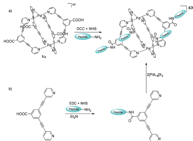
Fig. 29 (a) Direct peptide tethering to metallacage V'''_{Pd} and (b) initial ligand anchoring to the peptide, followed by self-assembly of metallacage V'''_{Pd} . Reproduced with permission from ref. 109. Copyright 2017, Royal Society of Chemistry.
