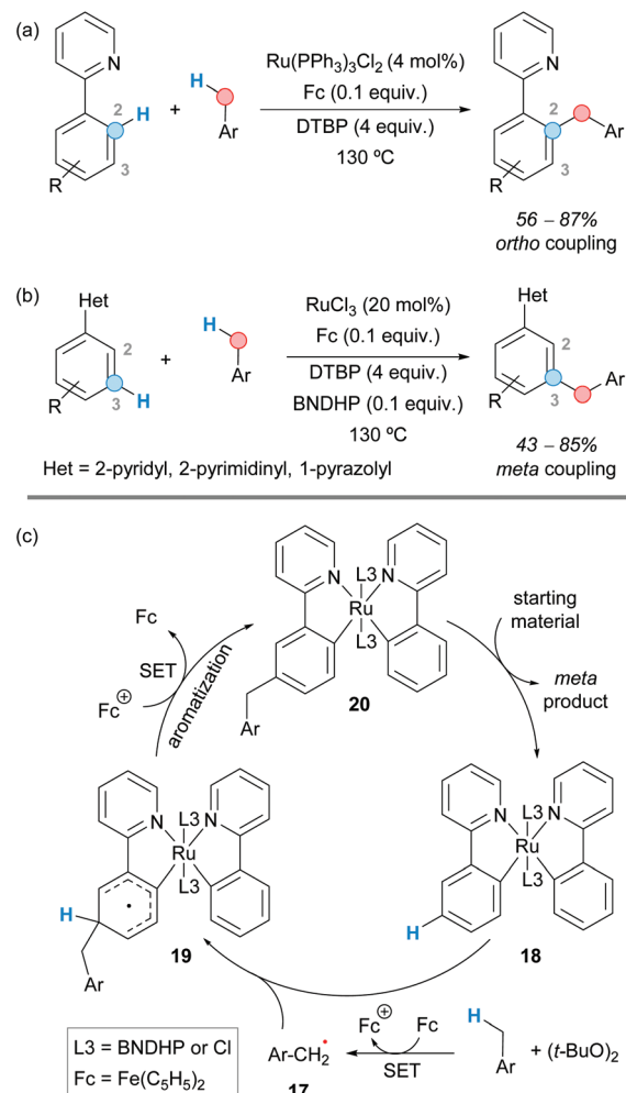
Scheme 11 Selective ruthenium-catalyzed ortho - and meta -benzylation of arenes and suggested catalytic cycle in the formation of the meta product.
