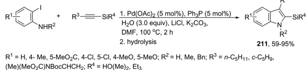
Scheme 172
