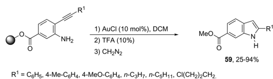
Scheme 53
