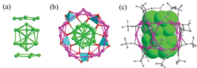
Fig. 19 X-ray structure of \text{Ag}_{48}(t\text{BuC}\equiv\text{C})_{20}(\text{CrO}_4)_7 . (a) Formation of the \text{Ag}_{25} shell by capping two silver pentagons on the \text{Ag}_{13} Ino decahedron on the top and bottom; (b) top view of the coordination of five equatorial \text{CrO}_4^{2-} anions linking the \text{Ag}_{23} cylinder and \text{Ag}_{25} shell; and (c) side view of the \text{Ag}_{23} cylinder encircled by the outer [\text{Ag}_{25}(t\text{BuC}\equiv\text{C})_{20}] shell. Adapted with permission from ref. 97. Copyright 2019, American Chemical Society.
