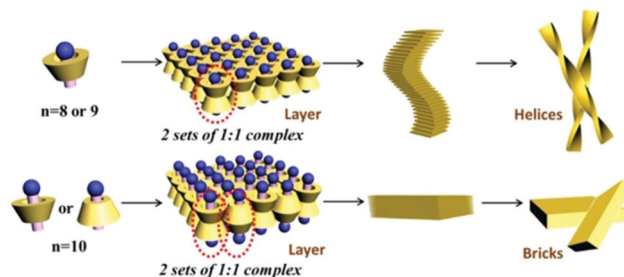
Fig. 14 Illustration of different complexation modes between long chain amines and β-CD. Upper: The amine head of CH 3 (CH 2 ) n-1 NH 2 (n = 8, 9) is toward the wider rim of β-cyclodextrin, which leads to the formation of helices. Bottom: The amine head of CH 3 (CH 2 ) n-1 NH 2 (n = 10) is toward both the narrower and wider rims of β-cyclodextrin, which leads to the formation of planar bricks. (Reprinted with permission from ref. 106. Copyright © 2018 Wiley-VCH.)
