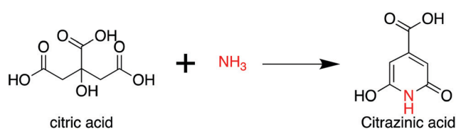
Scheme 2 The reaction of citric acid with ammonia.
