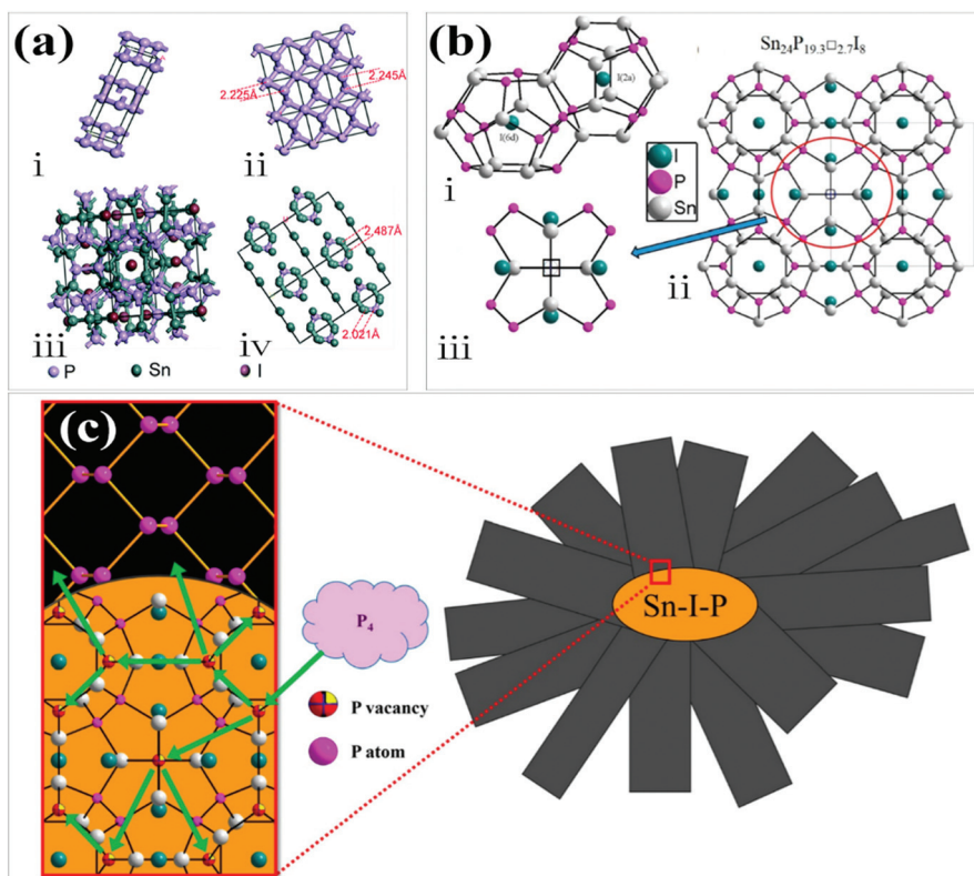
Fig. 6 (a) (i) BP unit cell, (ii) ring-like fragments of BP (viewed along the (020), (040) and (060) planes), (iii) the unit cell of Sn 24 P 19.3 I 8 and (iv) ring-like fragments of Sn 24 P 19.3 I 8 (viewed along the (600) plane). (b) (i) Pentagonal dodecahedra and tetrakaidecahedron frameworks formed by Sn and P atoms in the clathrate Sn 24 P 22-x I 8 and (ii, iii) the crystal structure of Sn 24 P 22-x I 8 . (c) Schematic of the proposed growth mechanism. Reproduced with the permission from ref. 32 and 33. Copyright 2017 The Royal Society of Chemistry and 2017 American Chemical Society, respectively.
