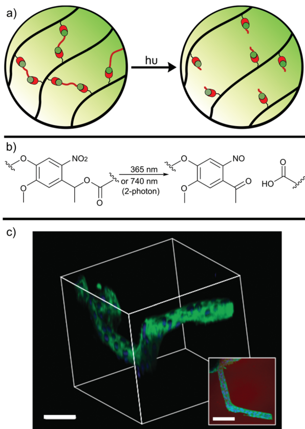
Fig. 14 (a) Schematic of a responsive hydrogel, where chemical crosslinks are broken in response to a light stimuli; (b) nitrobenzyl ethers undergo photocleavage in response to either single ( \lambda = 365 nm) or 2-photon ( \lambda = 740 nm) irradiation; (c) 3D patterning of channels in a PEG-based hydrogel by a combination of photodegradation and photo thiol-ene modification with RGD motifs, allowing the encapsulation and outgrowth of 3T3 fibroblasts. Inset is a top-down projection of the channels. Red – hydrogel; green – F-actin; blue – cell nuclei, scale bar 100 \mu\text{m} . Reprinted by permission from Springer Nature, Nature Chemistry , 'Cytocompatible click-based hydrogels with dynamically tunable properties through orthogonal photoconjugation and photocleavage reactions', C. A. DeForest and K. S. Anseth, 2011. 344
