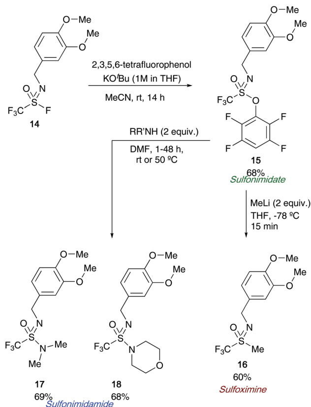
Scheme 4 Wright and Oehlrich's bench stable sulfonimidate from sulfonimidoyl fluorides, and further applications of sulfonimides.
