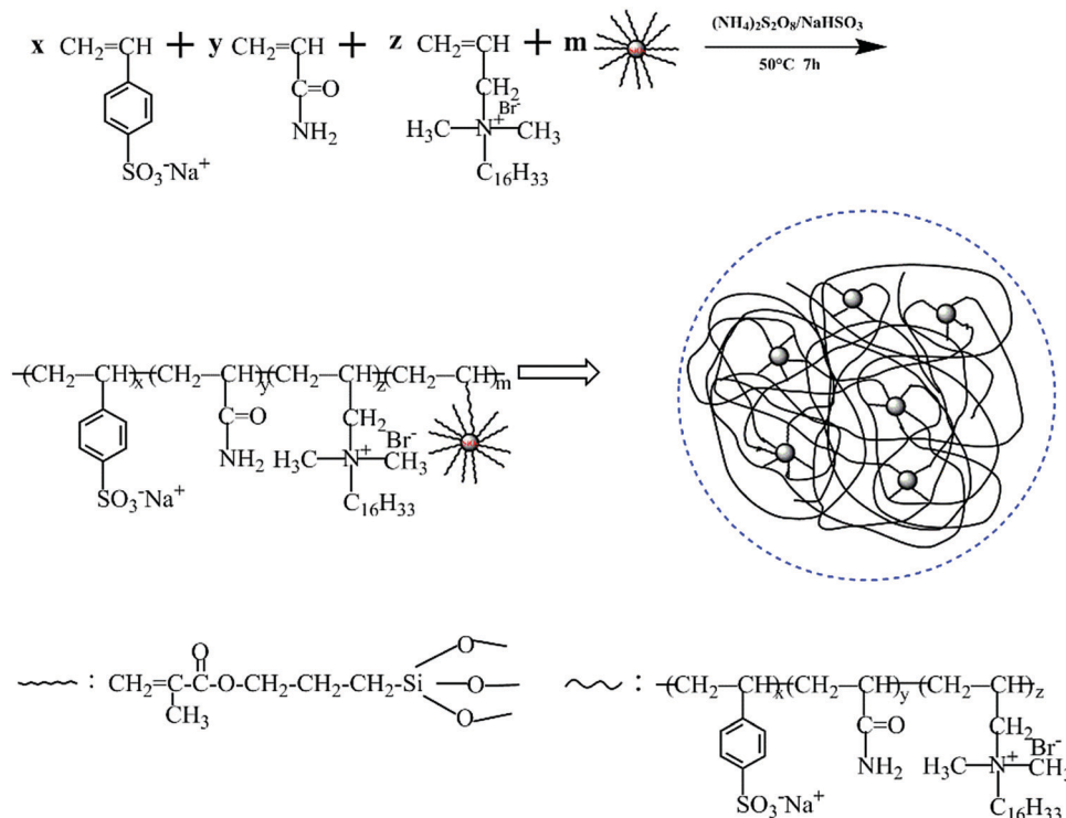
Fig. 3 Chemical route to the synthesis of PASD- SiO_2 .
