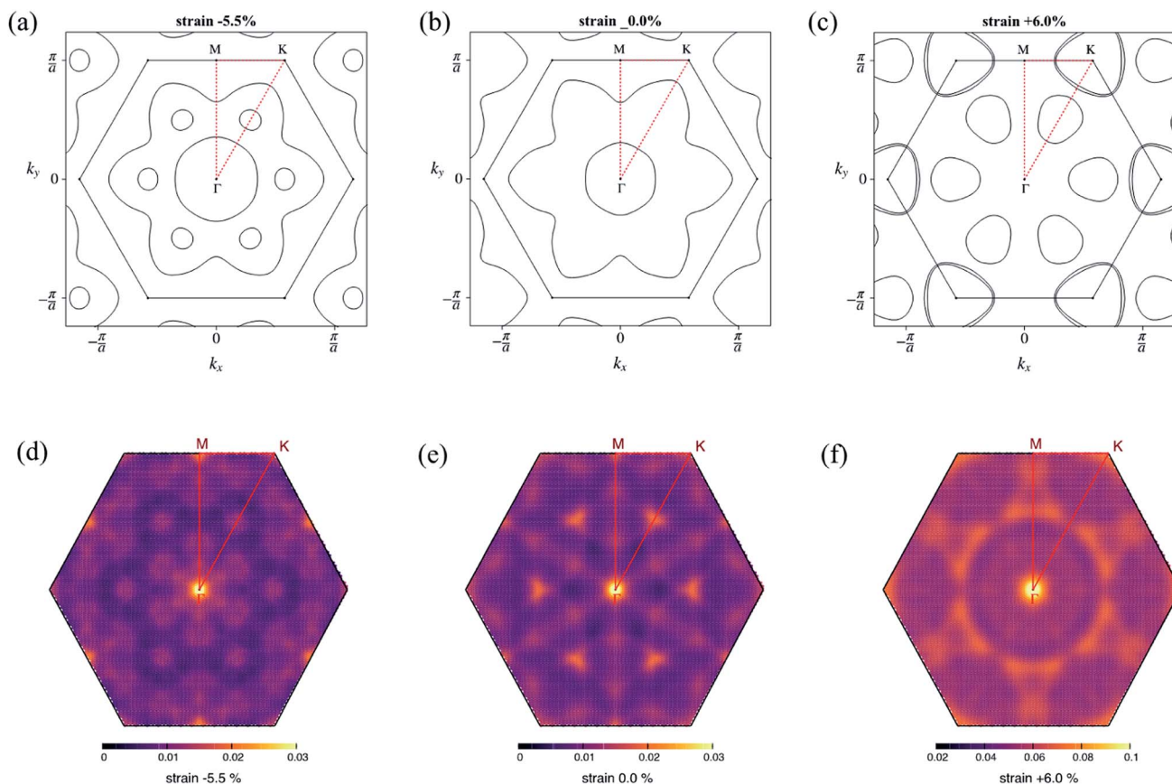
Fig. 2 Fermi surface and nesting function at zero strain (b) and (e), -5.5% of compressive strain (a) and (d) and +6.0% of tensile strain (c) and (f) corresponding to the equilibrium state and where the maximum T_c appeared. The order of the nesting function at +6.0% strain was larger than that of the zero or compressive strain case. Note that the range of the color scale in (f) differs from those in (d) and (e).
