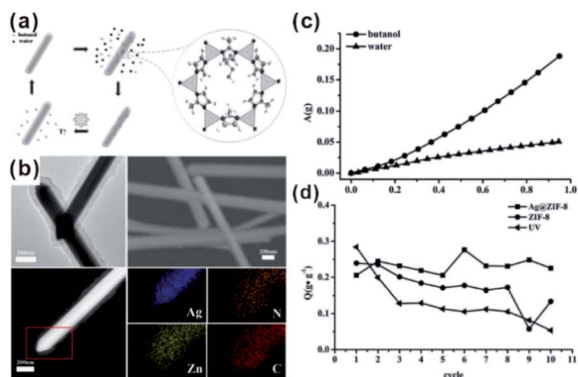
Fig. 15 (a) Scheme of a solar-light-driven adsorption/desorption process by core–shell Ag@ZIF-8 nanowires as adsorbents for butanol separation. (b) SEM profiles, TEM images, HAADF-STEM pictures, and EDX elemental mapping of single core–shell Ag@ZIF-8 nanowires. (c) Single-component adsorption isotherms of core–shell Ag@ZIF-8 nanowires toward butanol and water. (d) Comparison of butanol adsorption amount ( Q ) of different samples after 10 adsorption/desorption cycles. Reproduced with permission. 134 Copyright©2015 WILEY-VCH Verlag GmbH & Co. KGaA.
