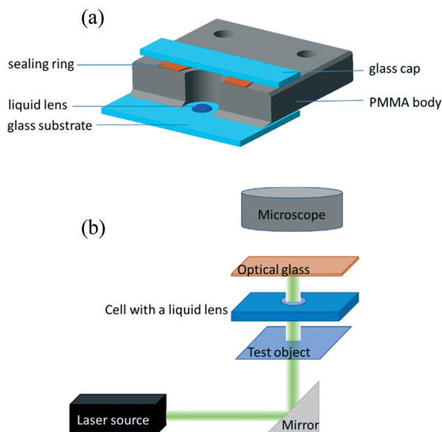
Fig. 1 (a) Schematic view of the liquid cell. (b) The experimental setup.
