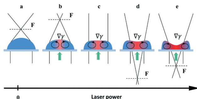
Fig. 2 Schematic illustration of the droplet reshaping by the thermocapillary forces induced with the laser beam. The axis shows the laser power increase. \nabla\gamma is the thermal surface tension gradient along the liquid interface. (a) The initial shape of the droplet (the laser is off); (b) the flattening of the droplet surface – the focal length increases (the laser is on); (c) the droplet with the flat surface – the focal length tends to infinity; (d) and (e) the formation of thermocapillary dimple in the droplet, negative focal length.
