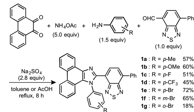
Scheme 1 Synthesis of phenanthroimidazolylbenzothiadiazoles 1a–g .
