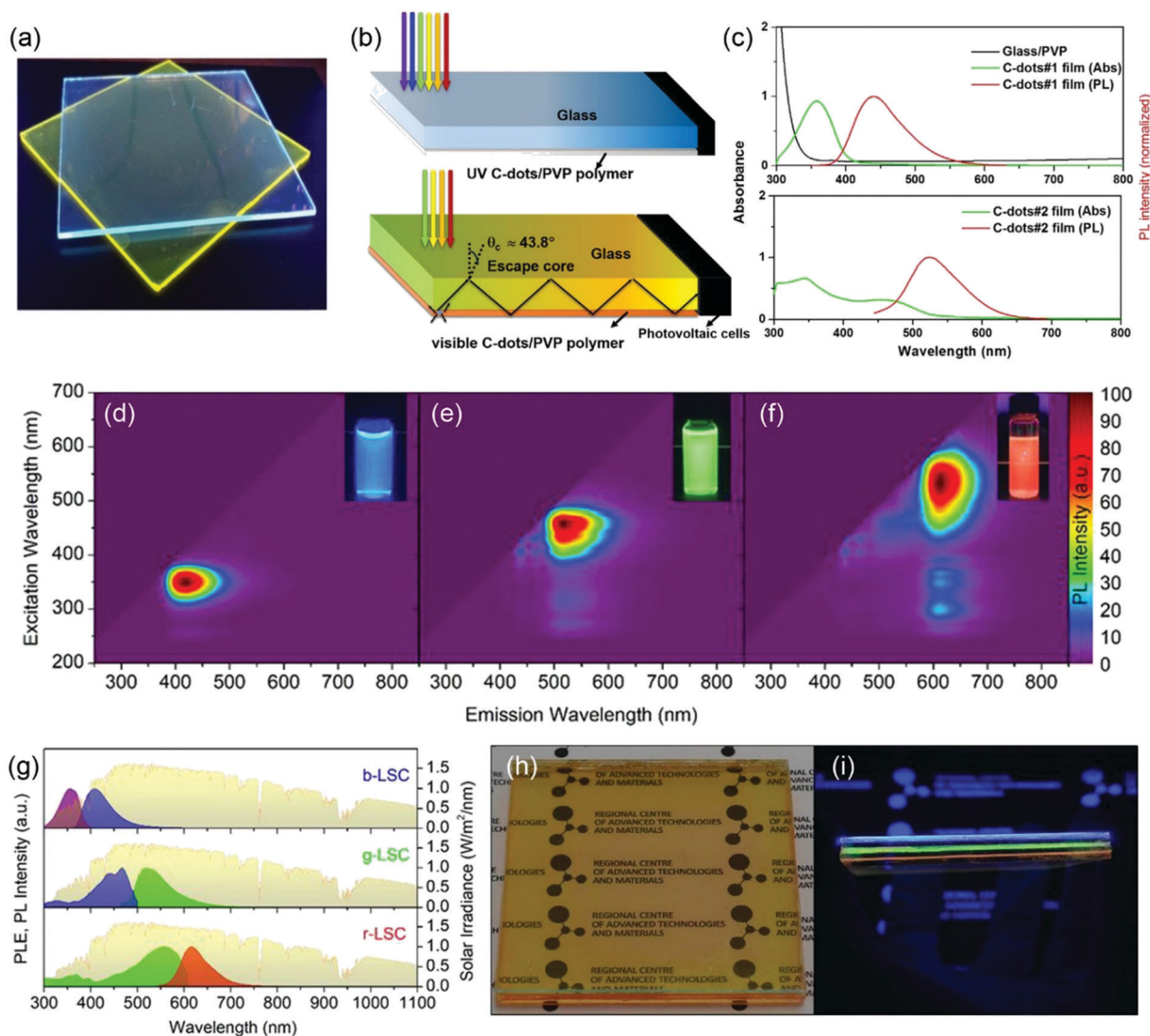
Fig. 13 Photograph (a) and schemes (b) of tandem thin-film LSCs based on UV C-dots (top) and visible NaOH treated C-dots (bottom). (c) The absorption and emission spectra of UV C-dots (#1, top) and visible NaOH treated C-dots (#2, bottom) based thin-film LSCs and absorption spectrum of PVP on a glass substrate. (d–f) Excitation–emission color maps of blue, green and red C-dots. Insets: Photographs of the corresponding C-dots solution under UV light. (g) PL excitation and emission spectra of individual LSCs based on blue, green and red C-dots compared with the AM 1.5 solar spectrum (in yellow). Photograph of the tandem LSC under daylight (h) and weak UV illumination (i). (a–c) Reproduced with permission from ref. 3. Copyright 2018 Elsevier. (d–i) Reproduced with permission from ref. 144. Copyright 2020 The Royal Society of Chemistry.
