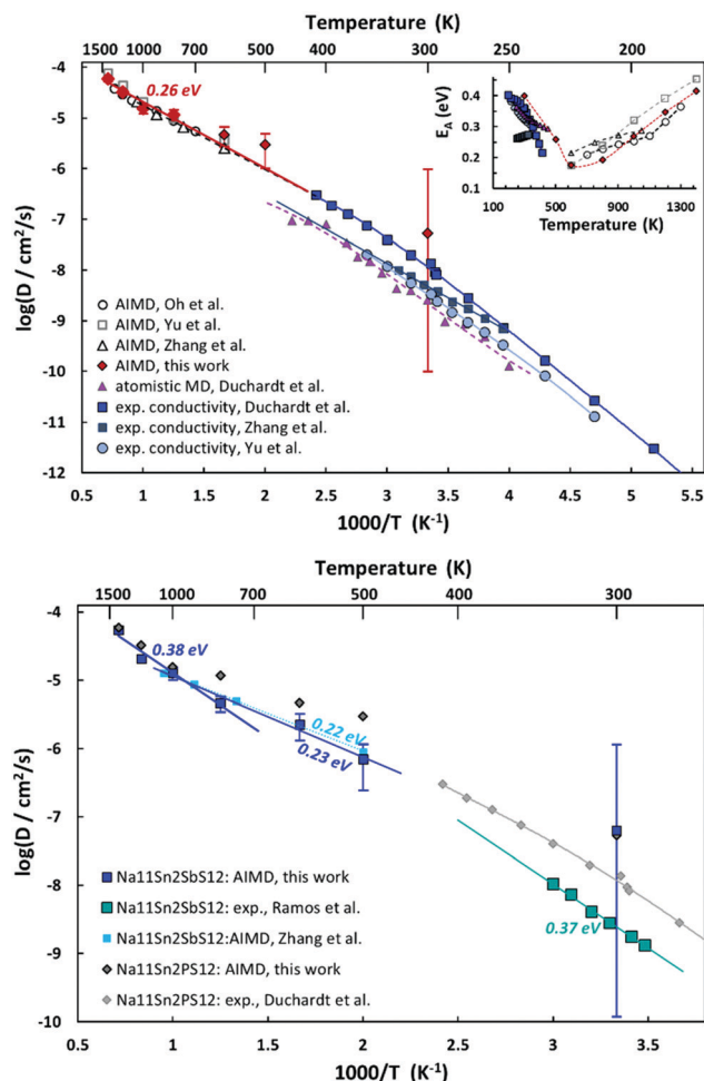
Fig. 12 Top: Arrhenius plot of AIMD-determined \text{Na}^+ diffusion coefficients for \text{Na}_{11}\text{Sn}_2\text{PS}_{12} (filled red diamonds) results from this work are compared to data from literature AIMD, empirical molecular dynamics simulations and experimental conductivity data. For the conversion of ionic conductivities a moderate degree of correlation with a Haven ratio of 0.5 has been assumed. The inset indicates the activation energies, E_a , derived from polynomial fits to the data in the main graph. Bottom: Arrhenius plot of AIMD-determined \text{Na}^+ diffusion coefficients for \text{Na}_{11}\text{Sn}_2\text{SbS}_{12} (dark blue squares) compared to AIMD (light blue) and experimental literature data (turquoise) as well as (in grey) selected data for \text{Na}_{11}\text{Sn}_2\text{PS}_{12} .
