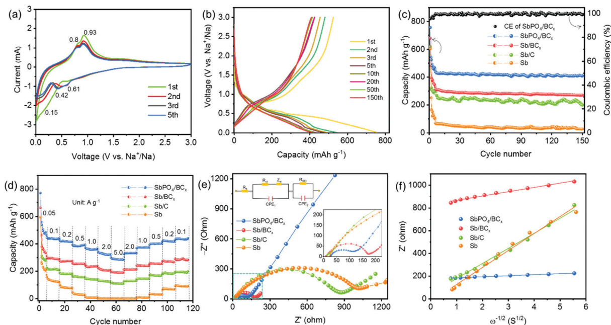
Fig. 5 (a) CV curves of the \text{SbPO}_4/\text{BC}_x electrode at a scan rate of 0.1 \, \text{mV} \, \text{s}^{-1} . (b) Galvanostatic charging/discharging curves of the \text{SbPO}_4/\text{BC}_x electrode at a current rate of 0.2 \, \text{A} \, \text{g}^{-1} over 3.0–0.01 V. (c) Cycle performance of the \text{SbPO}_4/\text{BC}_x , \text{Sb}/\text{BC}_x , \text{Sb}/\text{C} and \text{Sb} electrodes at a current rate of 0.2 \, \text{A} \, \text{g}^{-1} over 3.0–0.01 V. (d) Rate performance of the \text{SbPO}_4/\text{BC}_x , \text{Sb}/\text{BC}_x , \text{Sb}/\text{C} and \text{Sb} electrodes at various current rates from 0.1 to 5.0 \, \text{A} \, \text{g}^{-1} . Nyquist impedance plots and the magnified area (inset) in the range of 0–225 Ohm (e) and the corresponding relationship between the real part of the impedance ( Z_{\text{re}} ) and \omega^{-1/2} (f) of the \text{SbPO}_4/\text{BC}_x , \text{Sb}/\text{BC}_x , \text{Sb}/\text{C} and \text{Sb} electrodes.
