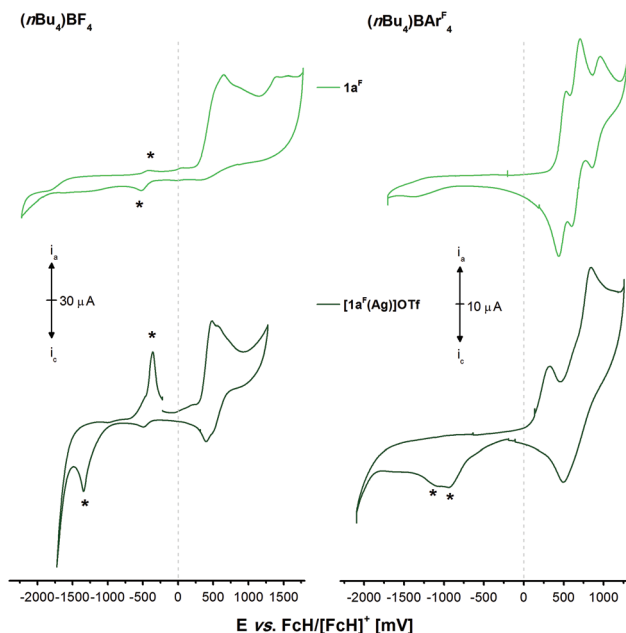
Fig. 9 Cyclic voltammograms of 1 mmol L −1 1a F (light green) and [1a F (Ag)]OTf (dark green) in 0.1 mol L −1 supporting electrolyte solutions ((nBu 4 N)BF 4 (left) and (nBu 4 N)BAr 4 F (right) in CH 2 Cl 2 ). Traces have been recorded at 100 mV s −1 (working electrode: glassy carbon, counter electrode: Pt wire) at room temperature. The second of three cycles are shown and asterisks (*) mark oxidation/reduction events which depend on prior oxidation in the first cycle ( cf. Fig. S66 and S67†).
