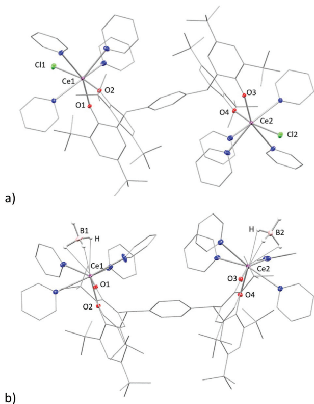
Fig. 3 Solid state structure of complex (a) 3-Ce (b) 3-Ce-BH 4 . Thermal ellipsoids are shown at 30% probability. All hydrogen atoms (except for BH 4 ) and solvents are omitted for clarity. Selected bond lengths in (a): Ln1–Cl1: 2.7789(6) Å (Ce), 2.7601(14) Å (Pr).
