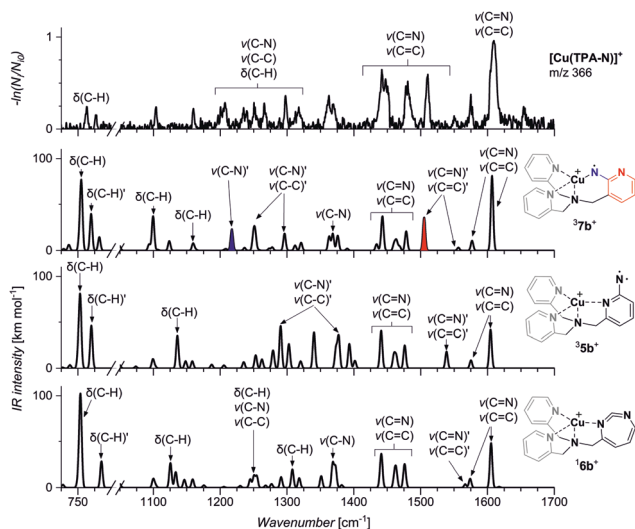
Fig. 3 Helium tagging infrared photodissociation spectrum of [\text{Cu}(\text{TPA-N})]^+ ( m/z 366) (top panel). Theoretical IR spectra of 3b , 35b and 16b were calculated for the optimized structures at the B3LYP/6-31+G* level and scaled by 0.97. \delta(\text{C-H}) , \nu(\text{C=C}) and \nu(\text{C=N}) correspond to the absorption bands in the pyridine rings whereas \delta(\text{C-H})' , \nu(\text{C=C})' and \nu(\text{C=N})' correspond to the absorption bands in the nitrene-pyridine ring.
