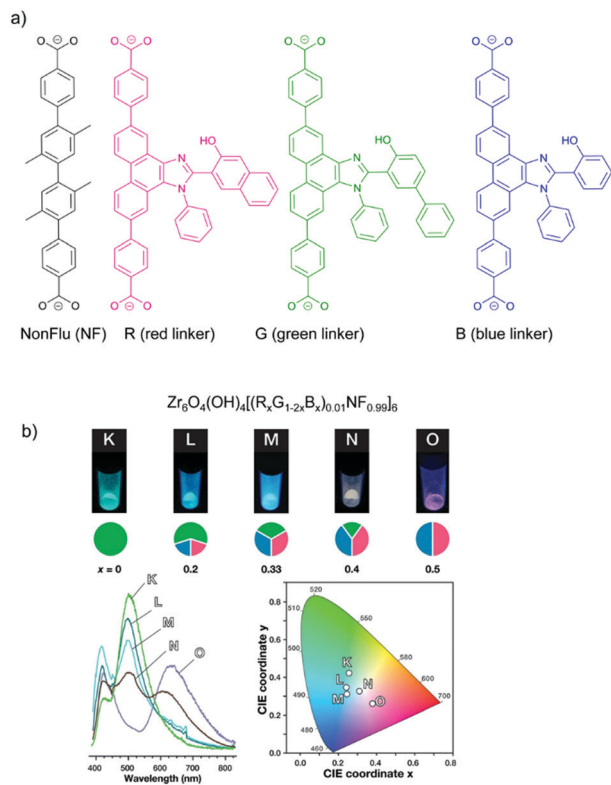
Fig. 4 (a) Solid solution formation with different RGB chromophore linkers in the UiO-type MOF [Zr 6 O 4 (OH) 4 (NonFlu) 6 ]. (b) Luminescence images (top), spectra (bottom left) and CIE chromaticity coordinates (bottom right) (under \lambda_{\text{ex}} = 365 nm irradiation) of the one to three-component RGB MOFs (with chromophore composition indicated in the cake diagrams below the luminescence images). Reproduced from ref. 61 with permission from the American Chemical Society, copyright 2019.
